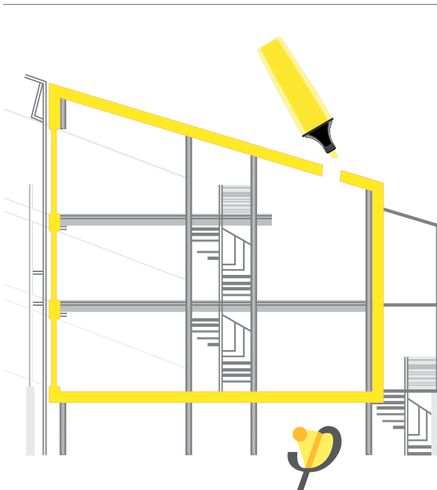
Fig. 7: Planning principle from the “plotter pen”. [www.passiv.de]
