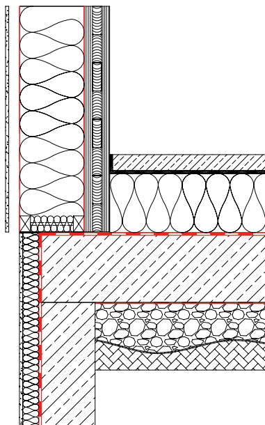
Base 1 – detailed condensation assessment necessary – see also chapter 02 “Highly heat-insulated external building components: floor slabs”
